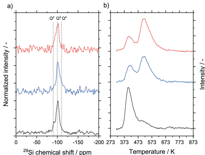
Fig. 7 a) ^{29}\text{Si} MAS NMR spectra and b) \text{NH}_3 -TPD measurement of untreated silica (black), hydrothermally treated at 393 K for 24 h (blue) and hydrothermally treated at 393 K for 100 h (red). All samples were calcined at 873 K before measuring as well as before reaction.
